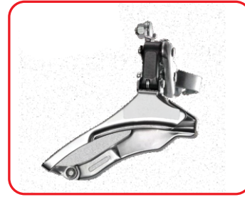
SBD-FD08 FRONT DERAILLEUR FRICTION DOWN PULL SUITABLE FOR 24/21 SPEED, CLAMP DIA-28.6MM /31.8MM TOP GEAR-48T, CAPACITY-22T FINISH-CP/UCP/ED
