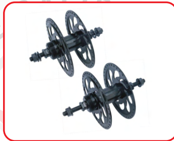
SBD-HBA21 STEEL HUB FREESTYLE SPOKE HOLES 36H/48H/68H, SPOKE DIA-2MM FINISH-ED
