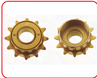
SBD-SF1201 TEETH-12T SIZE 1/2"X1/8"X12T FINISH-BLACK/BROWN/CP
