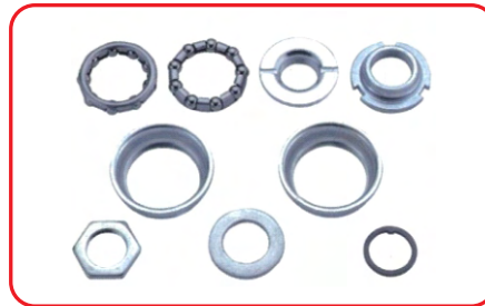
SBD-BF09 BB FITTING AMERICAN TYPE SET OF 9 PCS, THREAD-15/16"24TPI(RH) AND 7/8X24TPI (LH) BALL RETAINER-5/16"X9BA FINISH-BLACK/UCP
